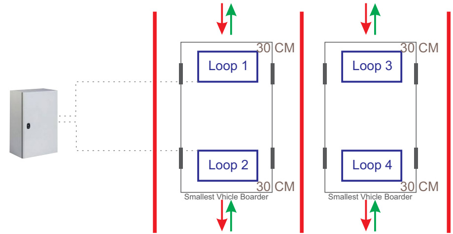
Separate Entry/Exit or Double use direction
