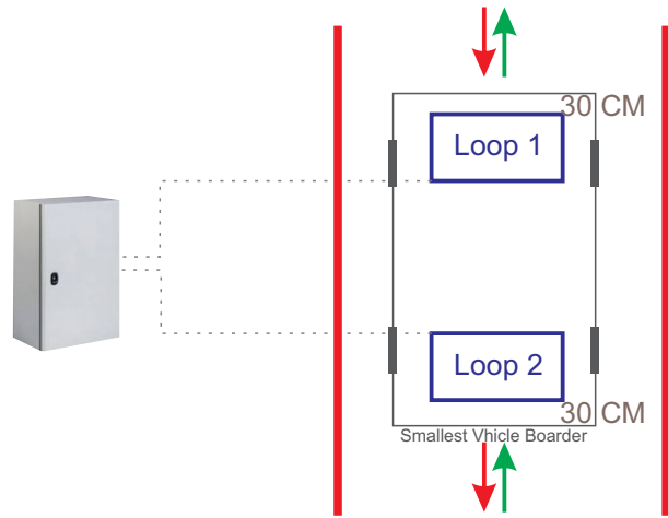
Single Lane Installation
