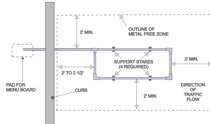
Magnetic loop accurate positioning (Good Practice)
