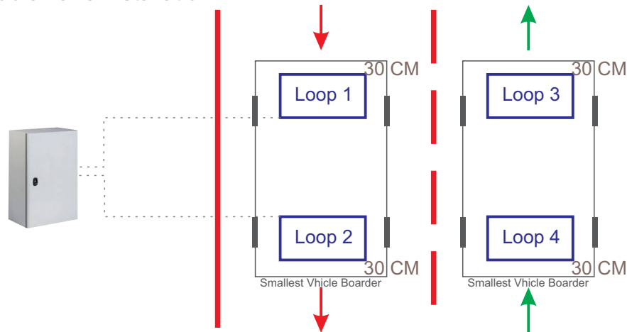
Double Lane Installation
